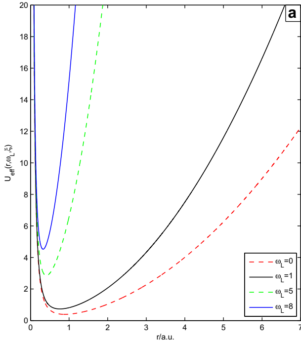
Fig. 1 The KG effective potential function for (a) \omega_L \neq 0 , \xi = 0 and (b) \omega_L = 0 , \xi \neq 0 . Here M = c = k = 1 .
