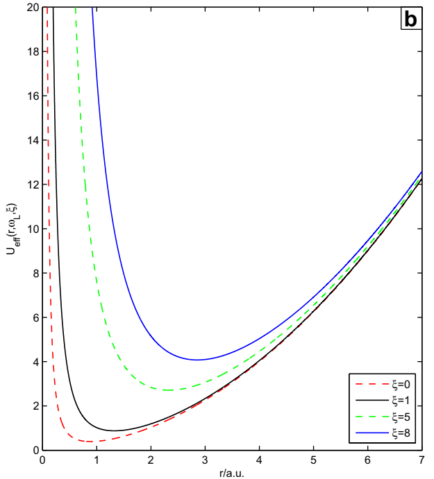
Fig. 1 The KG effective potential function for (a) \omega_L \neq 0 , \xi = 0 and (b) \omega_L = 0 , \xi \neq 0 . Here M = c = k = 1 .
