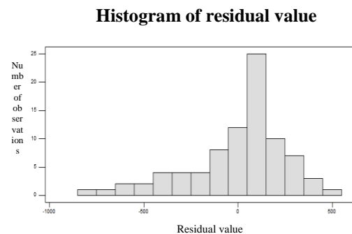
Figure 7. Histogram of residual value
