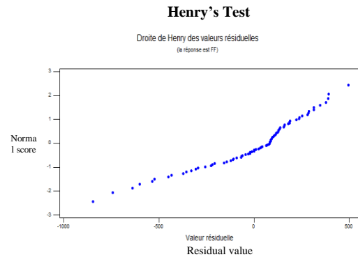
Figure 6. Henry's straight line test
