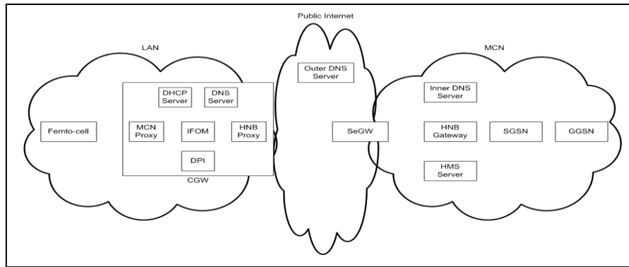
Figure 3. MCN nodes and CGW functional components
