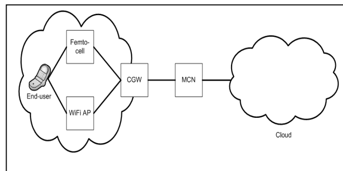
Figure 1. CGW Topology
